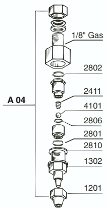
VALVOLA INIEZ. A SFERA fino a 20 l/h BALL INJECTION VALVE up to 20 l/h
