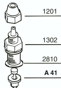
VALVOLA KALRETZ KALRETZ VALVE
